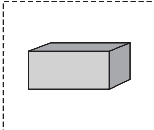
Cuboid
