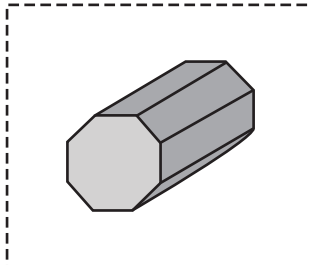
Octagonal prism
