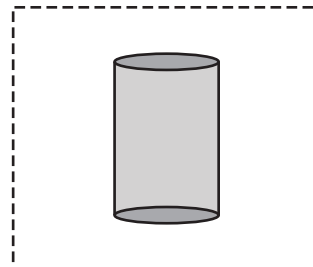
Cylinder
