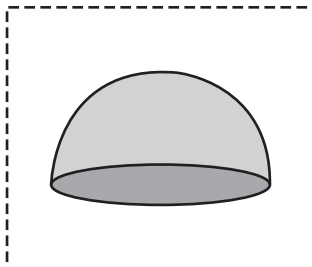
Hemisphere
