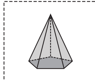
Pentagonal pyramid
